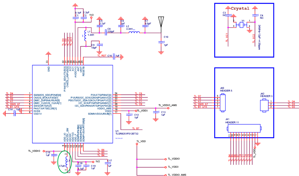
Figure 16- 2 Schematic for TLSR8251F512ET32
