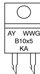
TO-220AC CASE 221B PLASTIC
