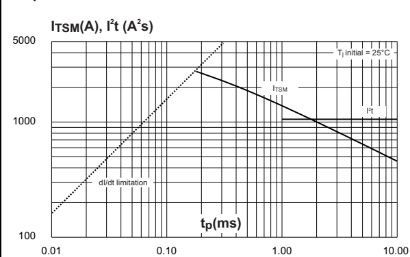
Figure 6. Non-repetitive surge peak on-state current for a sinusoidal pulse with width t_p < 10\text{ ms} , and corresponding values of I^2t
