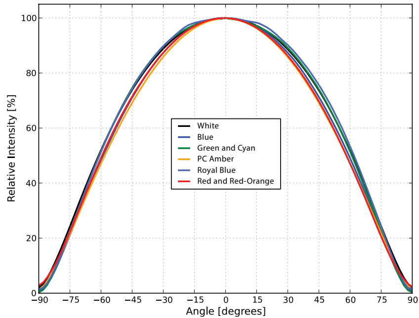
Figure 5a. Typical radiation pattern for LUXEON CZ Red, Red-Orange, PC Amber, Green, Cyan, Blue, Royal Blue and White at 350mA, T_j=85^{\circ}\text{C} .
