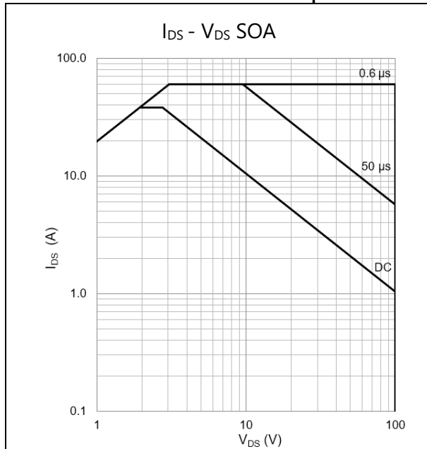
Figure 13: Safe Operating Area @ T_{case} = 25^{\circ}\text{C}
